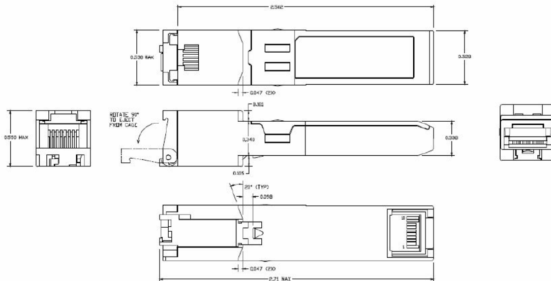
Figure 2. GS-Tx mechanical dimension
